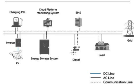
System Topology
